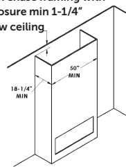
Framing to ceiling with front or side vents
