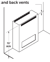
Minimum enclosure with front and back vents
