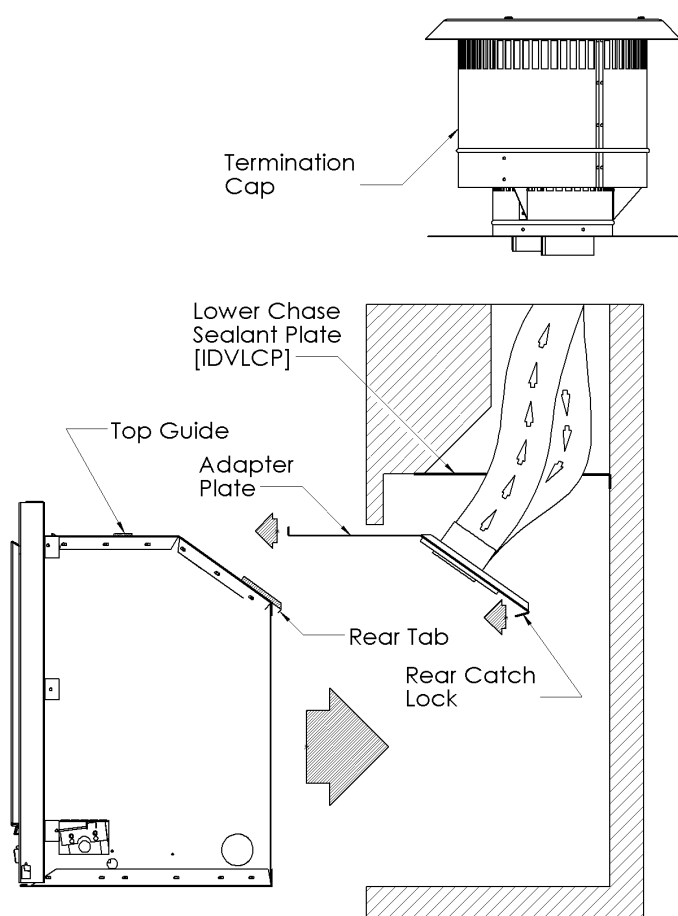
Fig. 2 - Base unit chimney venting install.
