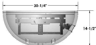
FPB30TBT / FPB30SGT 30" Bowl
