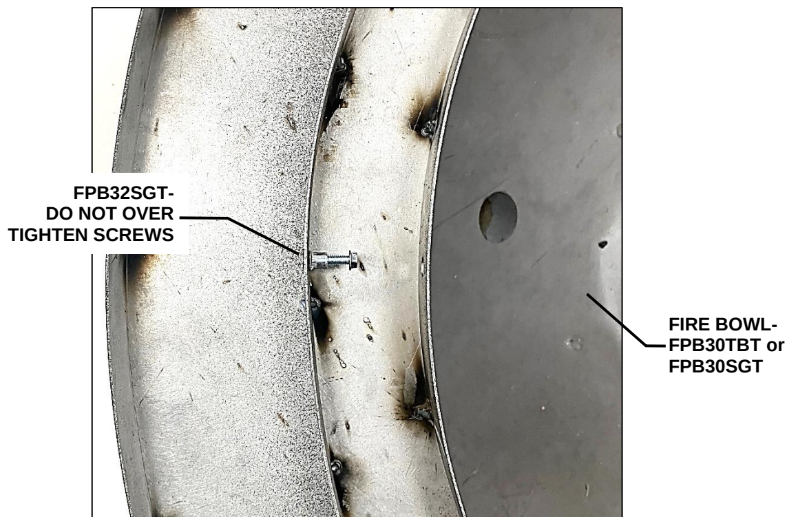
- BOTTOM VIEW OF TRIM RING INSTALLED ON BOWL -
