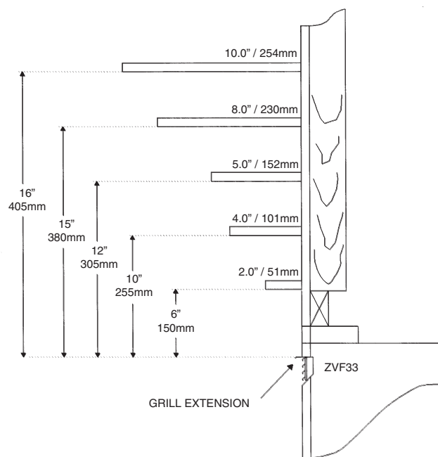
FIGURE 8 – Mantel Clearances.
