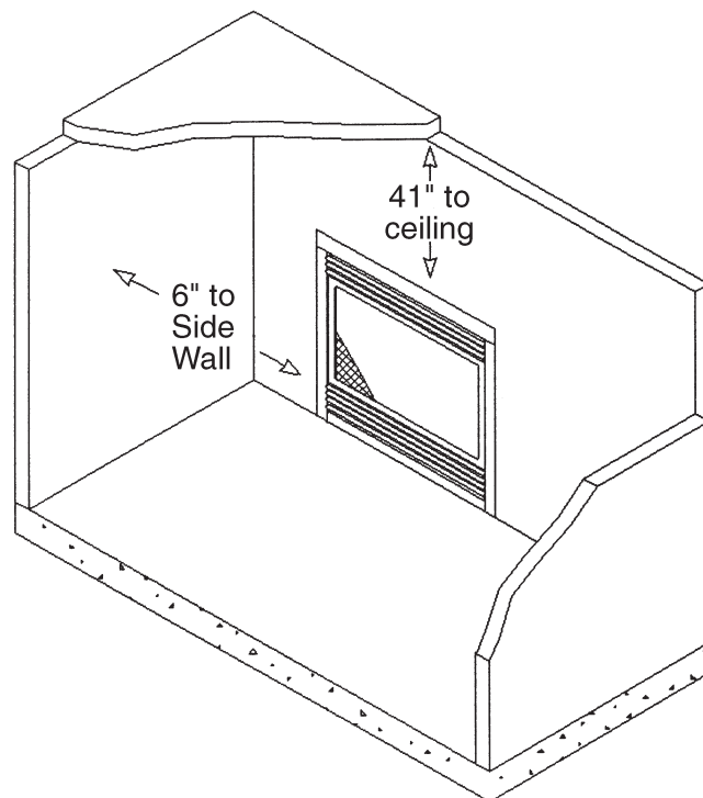
FIGURE 7 – Minimum Clearances - Top and Sides of Room Heater to Ceiling and Walls.
