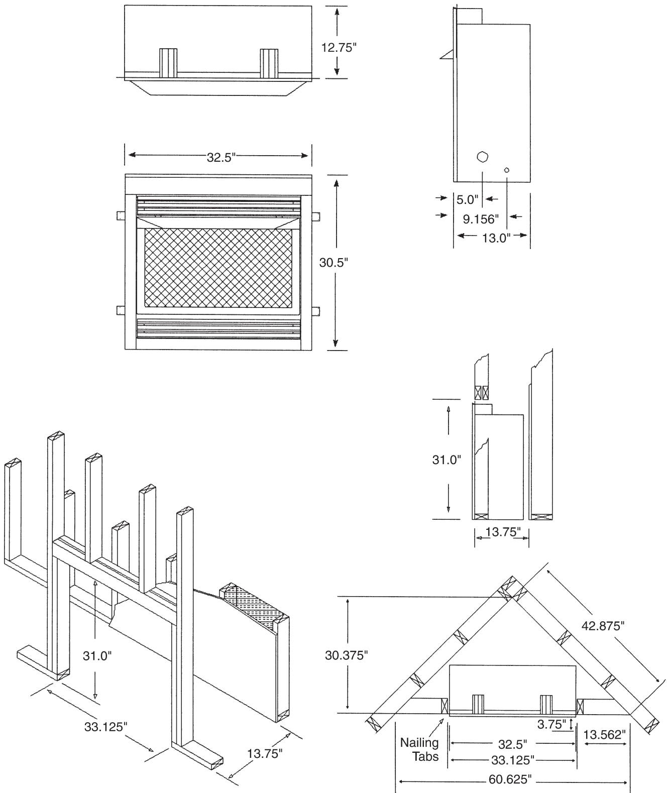
FIGURE 1 – ZVF33
