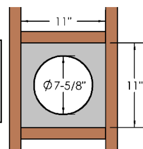
Framing for Horizontal Vent Termination (See Installation of Side Wall Venting Section)
