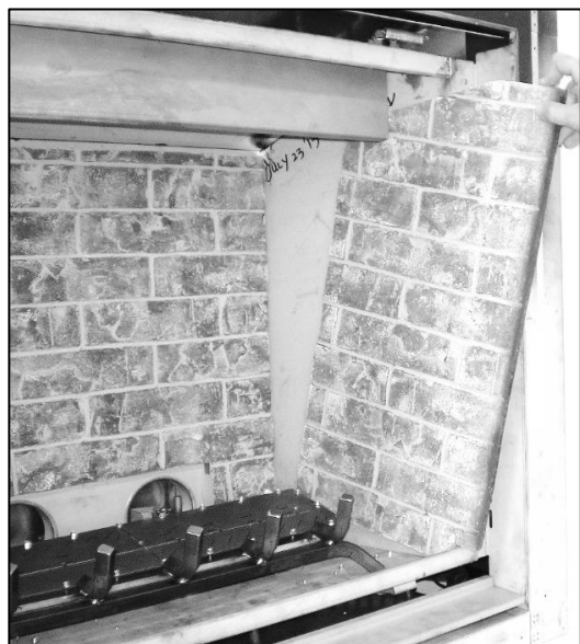
Step Three: Tilt and slide left and right Side Liners into place.
