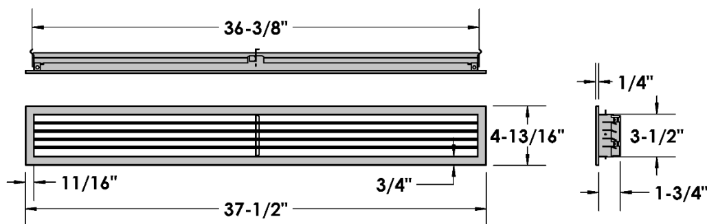
TOP VIEW
