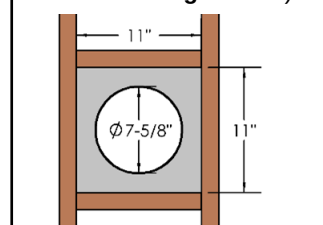
Fig.1 Framing for Horizontal Vent Termination (See Installation of Side Wall Venting Section)
