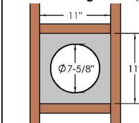
Fig.1 Framing for Horizontal Vent Termination (See Installation of Side Wall Venting Section)
