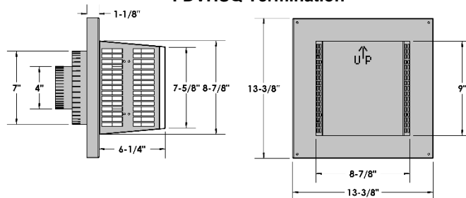
FDVHSQ Termination
