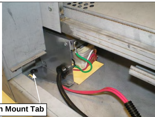
Set fan onto Mount Tabs inside fireplace.
