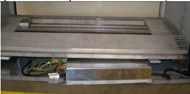
Remove Glass Doors from both sides of fireplace. Remove UHS Box from bottom of fireplace.
