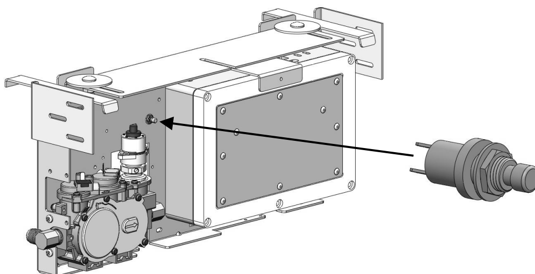
Remote Control Pairing Button
