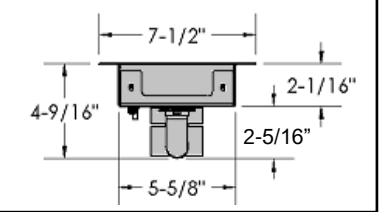
END VIEW- ALL BURNERS
