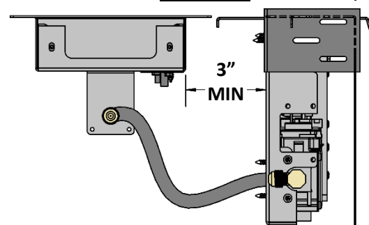
OBUEM2 Box Minimum Side Clearance from Burner Tray
