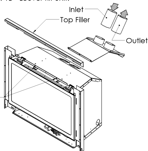
Fig. 3 - Remove top filler to install venting adapter.
