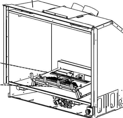
Base Unit (As Shipped)
