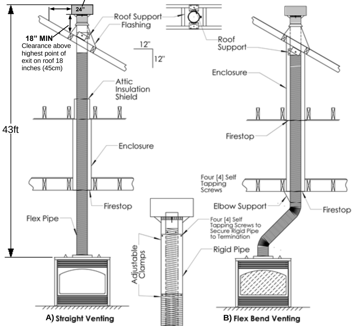
A) Straight-through roof support configuration; B) Flex bend configuration; C) Termination mounting
