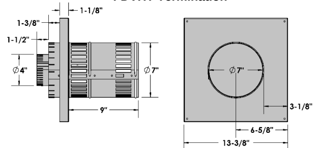
FDVHSQ Termination
