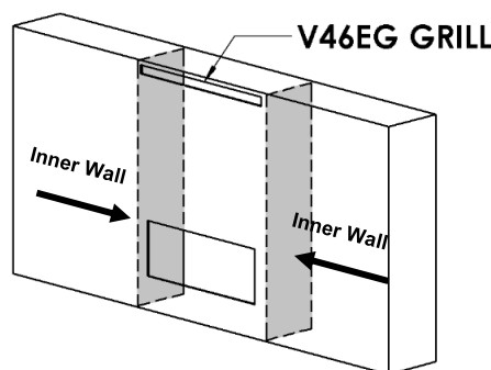
Optional Additional Rear Grill- Must be in the same Pressure Zone (Room / Area)
