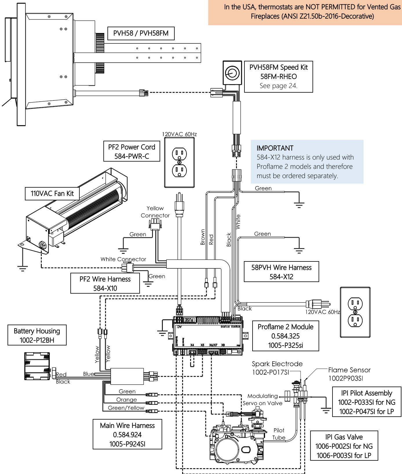
Figure 18 - Power Vent connection to Proflame 2 system with sample Fan Unit.
