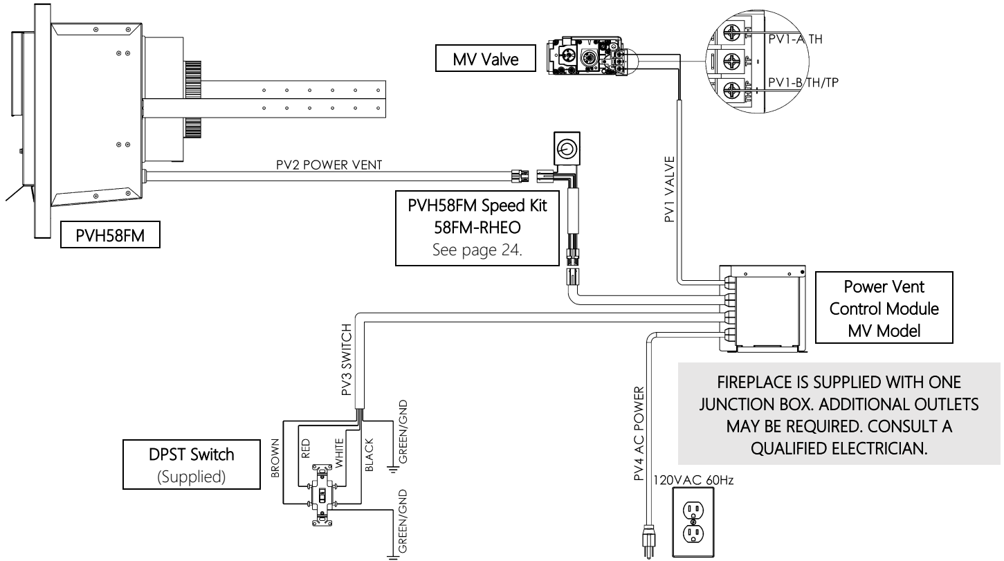
Figure 14 - Connecting Power Vent to a Millivolt system.
