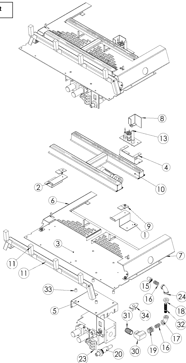
IDV33 / IDV43 Insert Burner Component List
